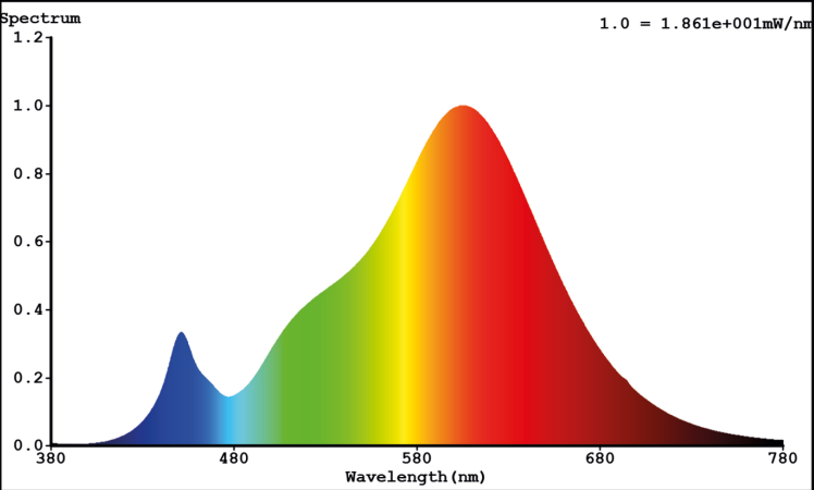
Spectral Distribution
