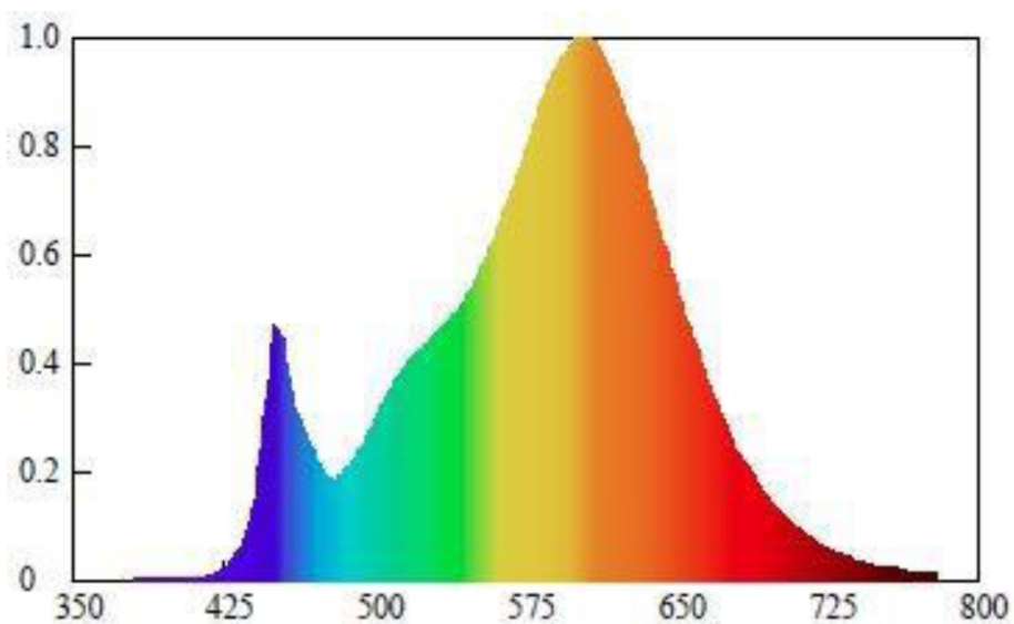
Model No.: 961912 Spectral Distribution
