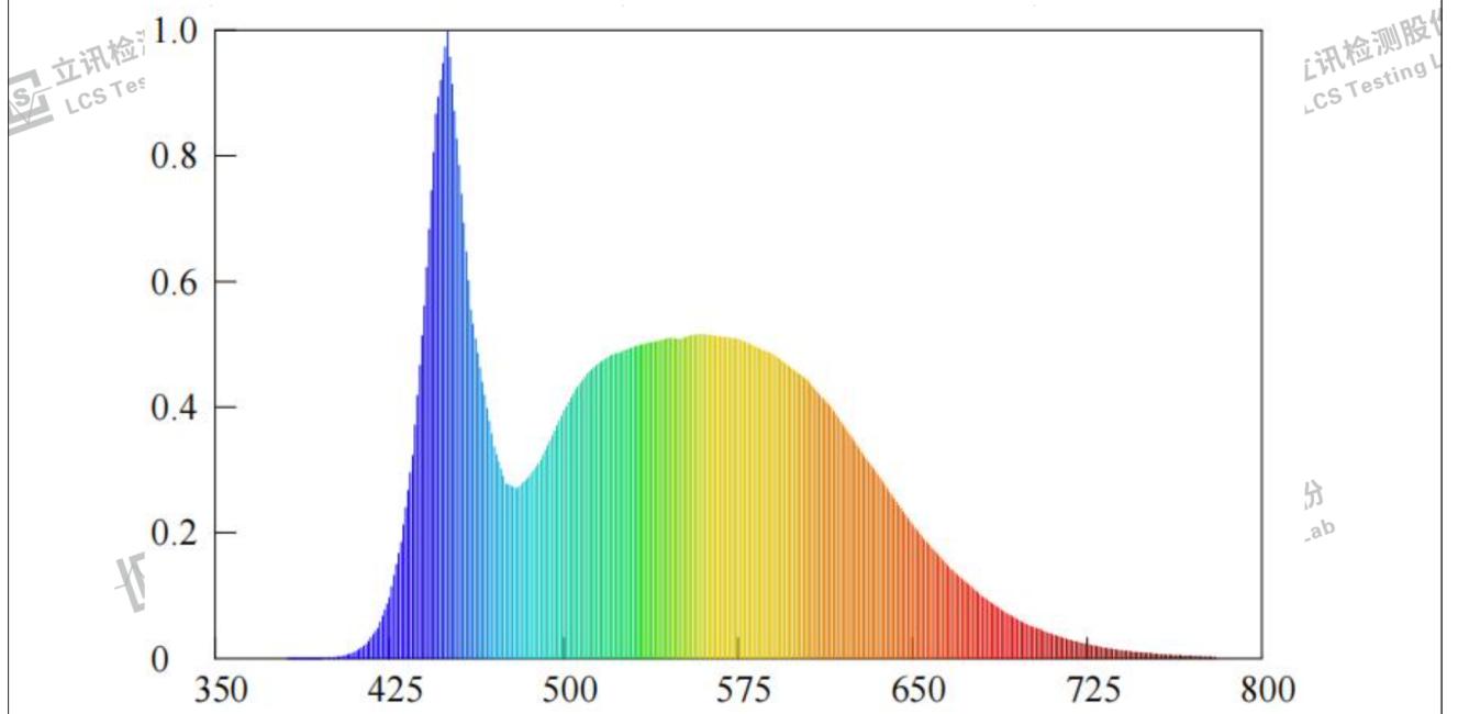
Spectral power distribution(6000k)
