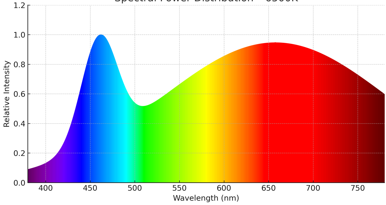
Spectral Power Distribution - 6500K
