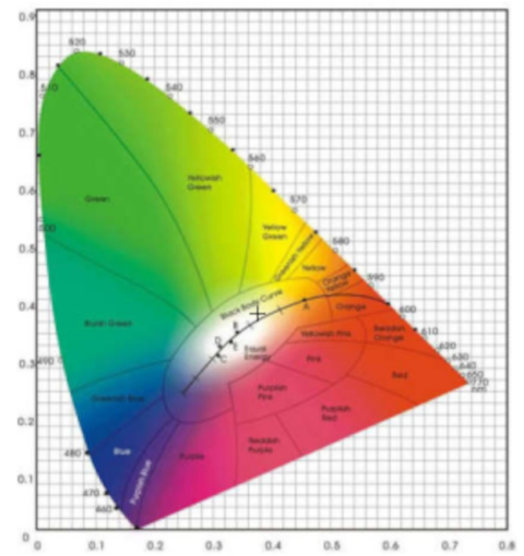
CIE1931
