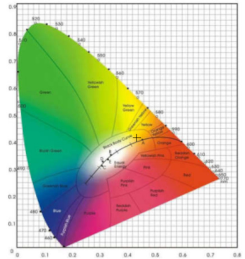
CIE1931
