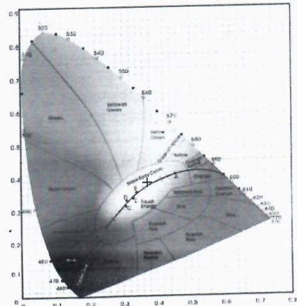
CIE1931
