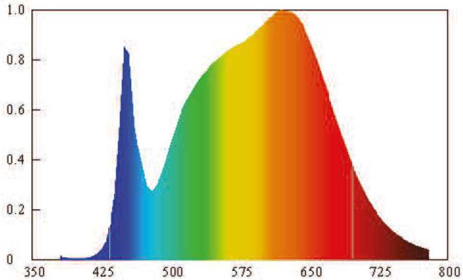
Spectral power distribution
