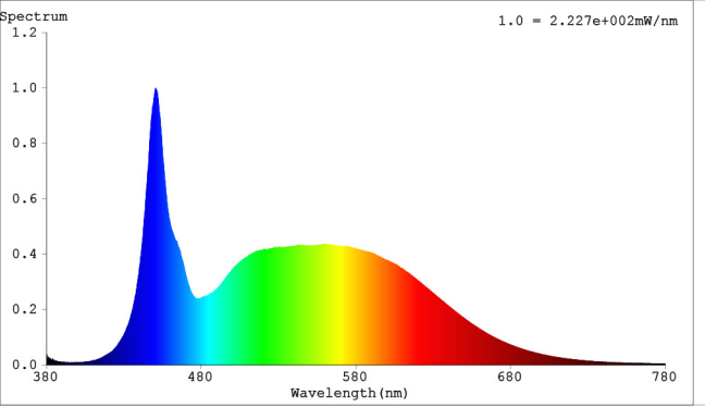
Spectral Distribution
