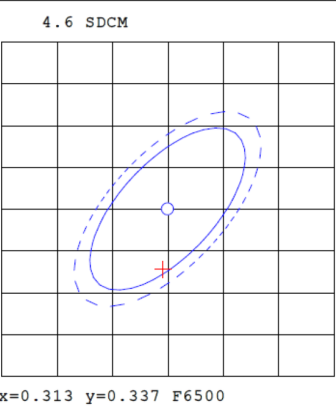
SDCM Chromaticity Diagram
