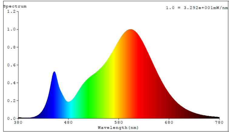
Spectral Distribution
