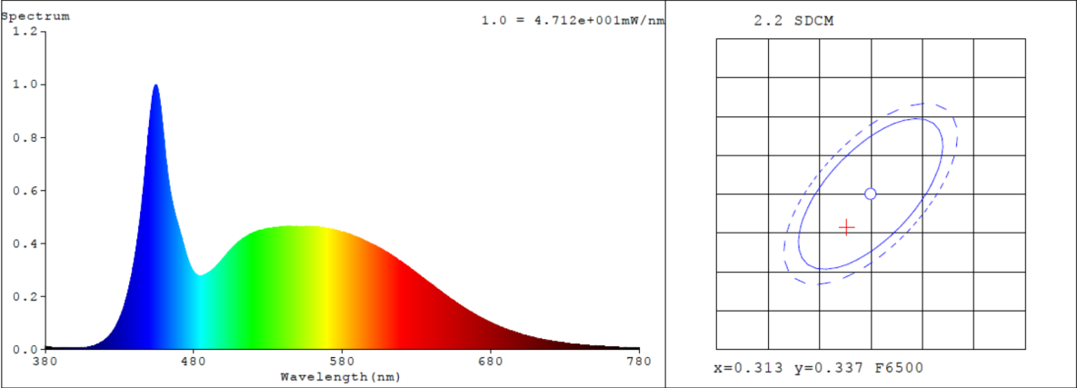
Spectral Distribution
