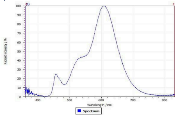
Spectrum of LED module
