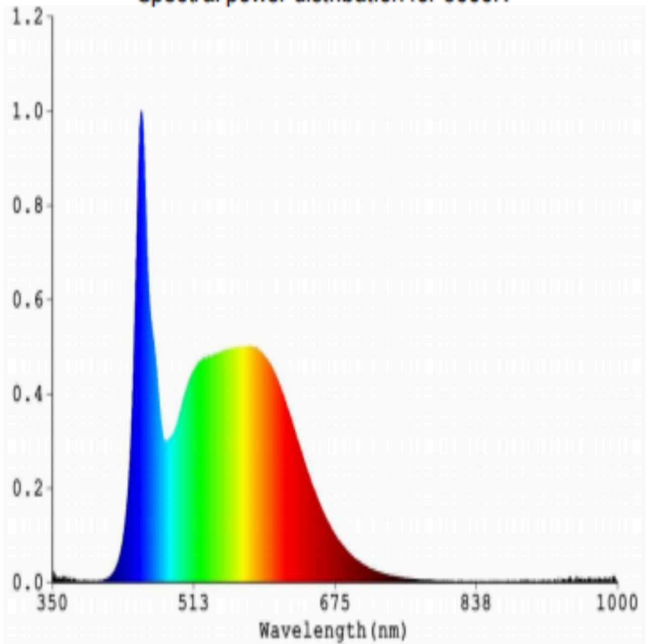
Spectral power distribution for LEDs
