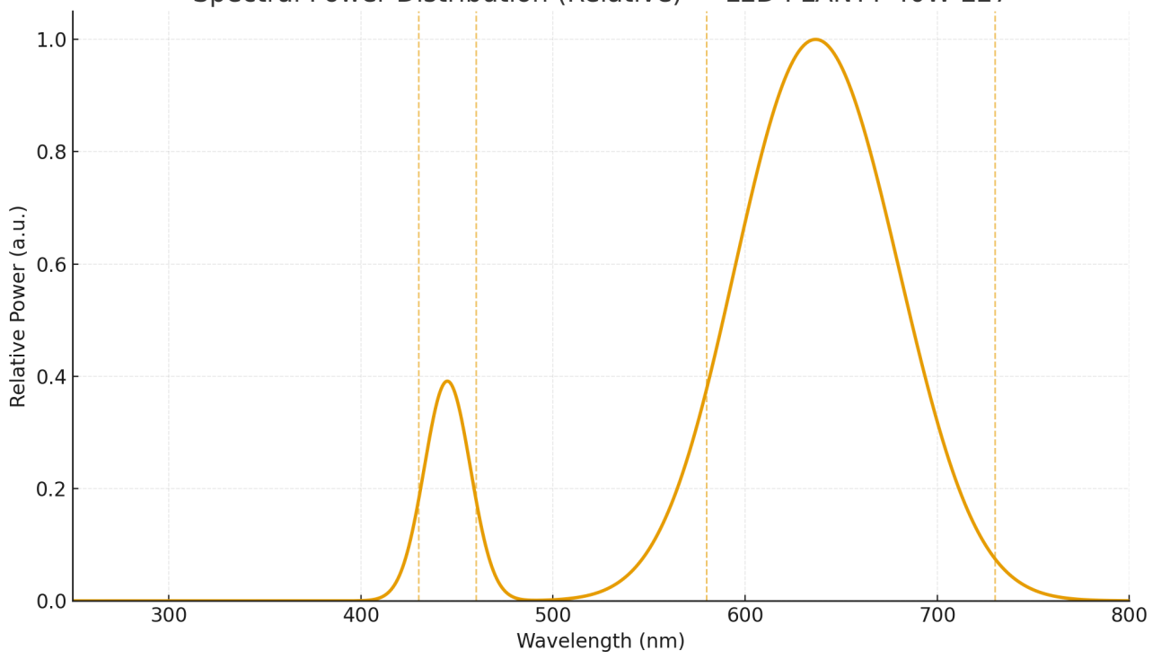
Spectral Power Distribution (Relative) — LED PLANTY 40W E27
