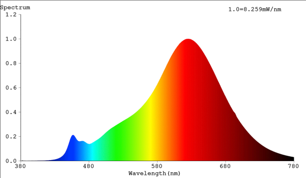
Spectral Distribution
