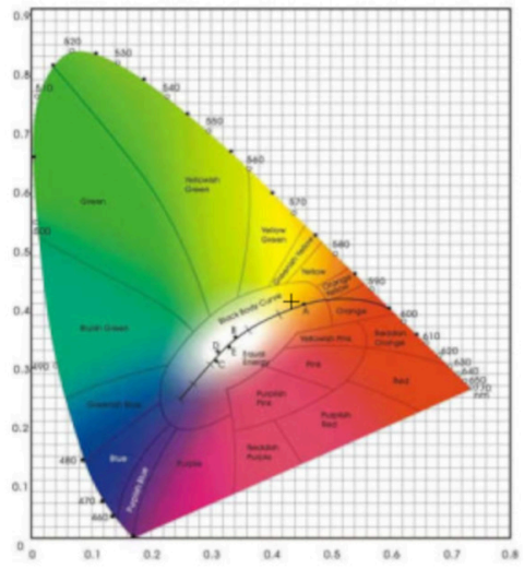
CIE1931
