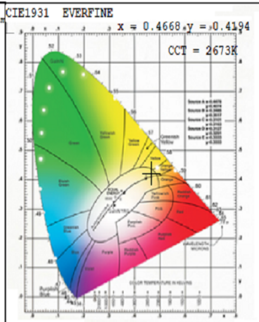
CIE1931 Chromaticity Diagram
