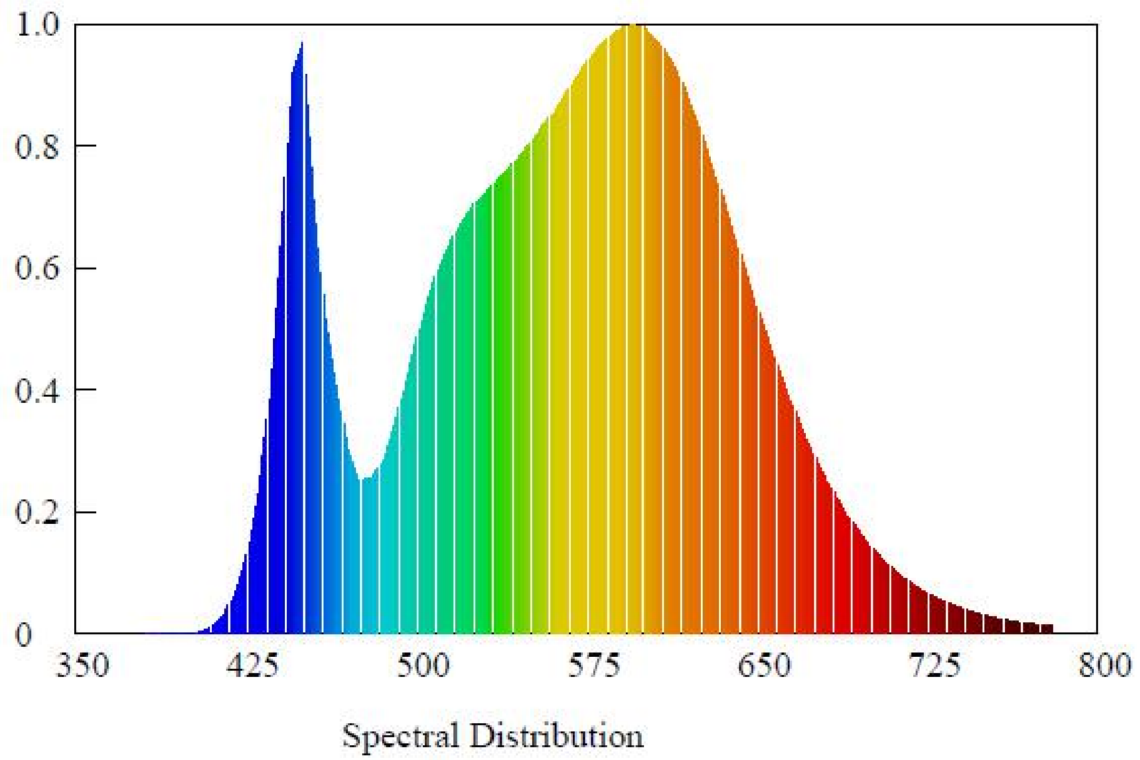
Spectral power distribution (4000K)
