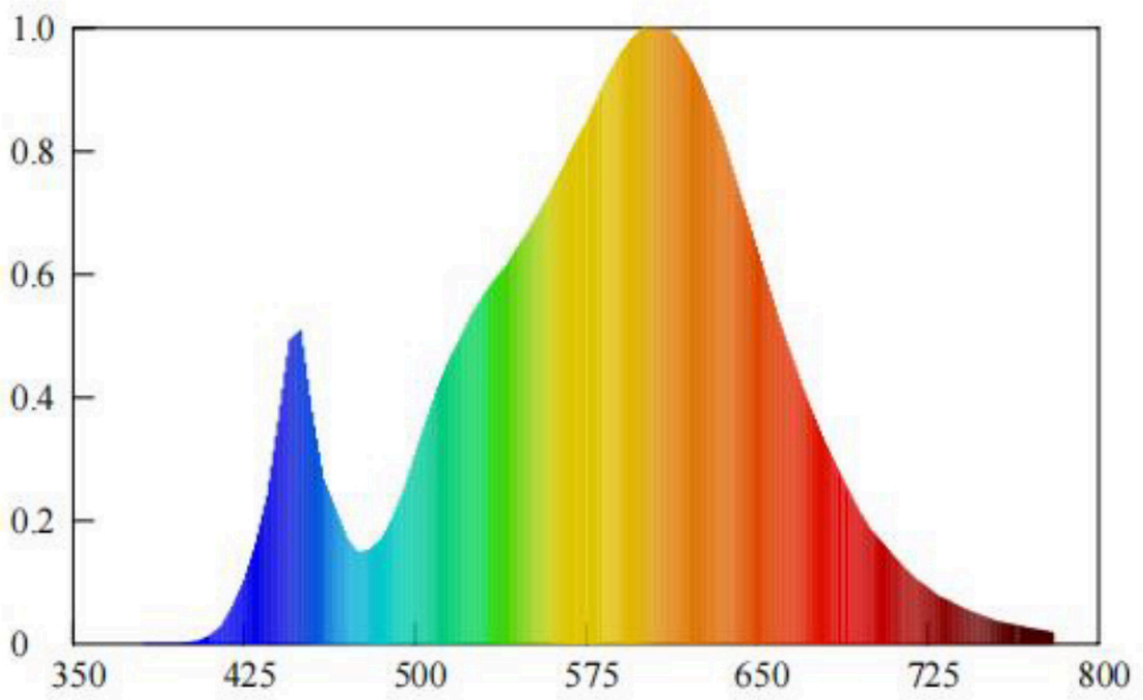
Spectral Distribution
