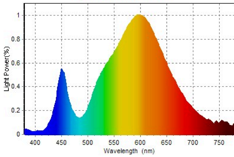
Spectral Distribution Curve □
