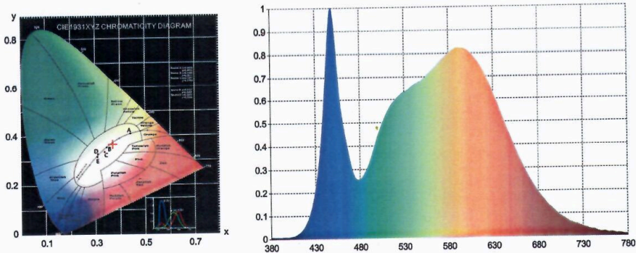
CIE1931 Chroma Figure
