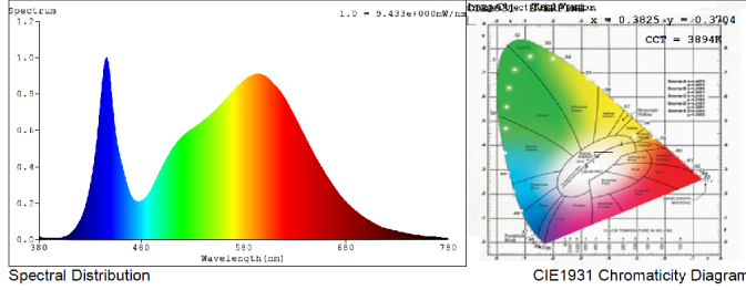
Spectral Distribution
