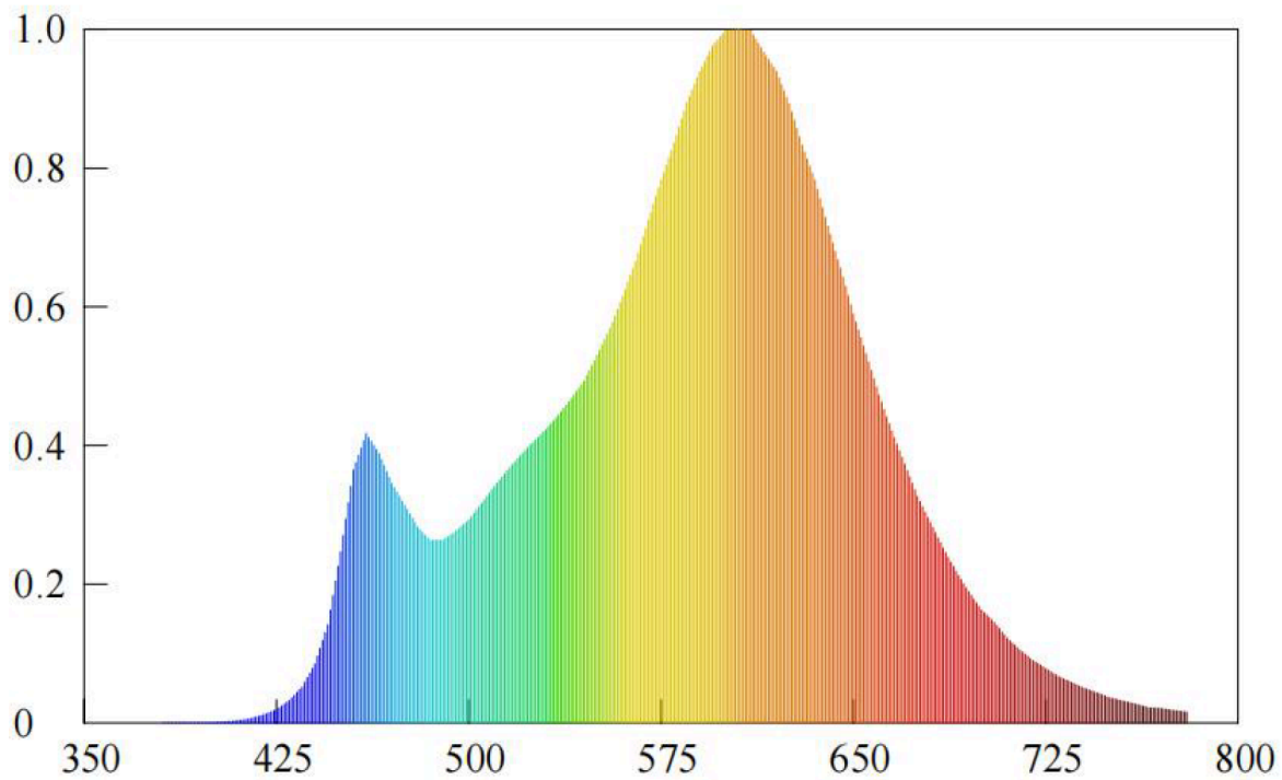
Spectral power distribution(5W)
