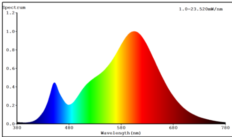
Spectral Distribution
