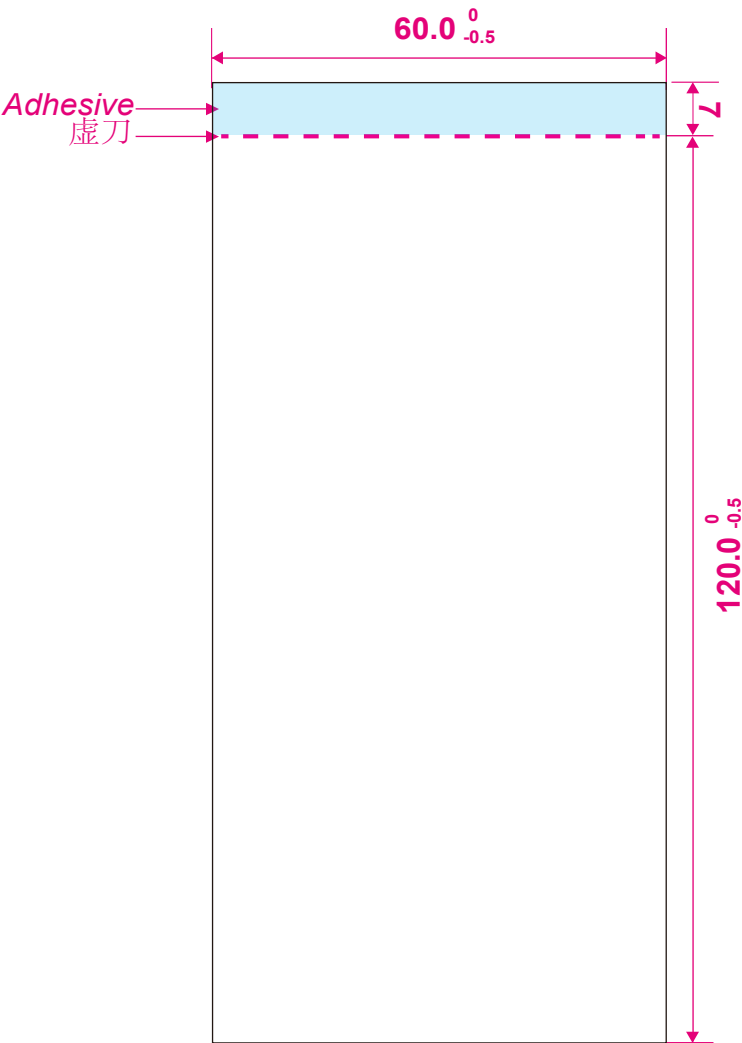
Back view
